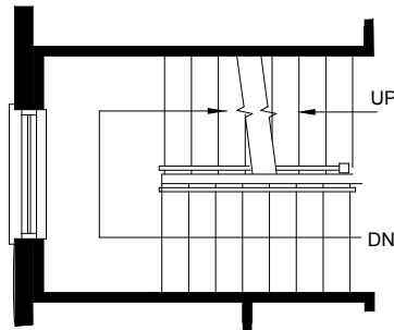
Second Floor Stairs for Loft Plan
